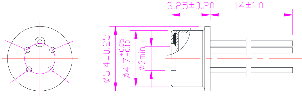
BOTTOM VIEW
